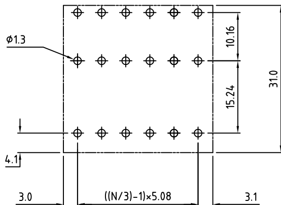
PCB Layout
